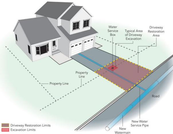
Trenchless water services installation: Driveway restoration without sidewalk
